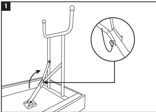
1. Detach table and unfold legs. Secure with metal pin.
