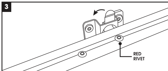
3. Align red rivets to latches and slide the table into place. Lock the latches into position by rotating to center.
